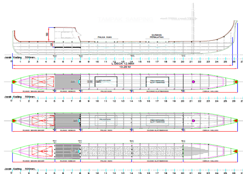
Figure 2. Sandeq Construction
