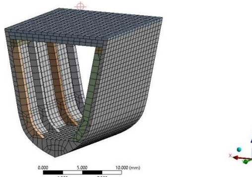
Figure 3. FE Model and Mesh
